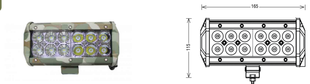
LED 3W* / 36W* / 9-32V / Flood / 12V~1912Lm** / 3600Lm* / ECE R10
